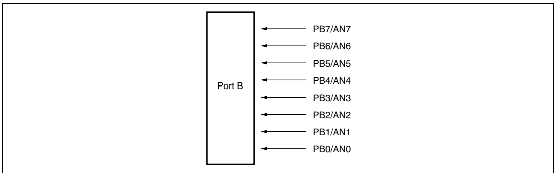
Figure 9.8 Port B Pin Configuration
