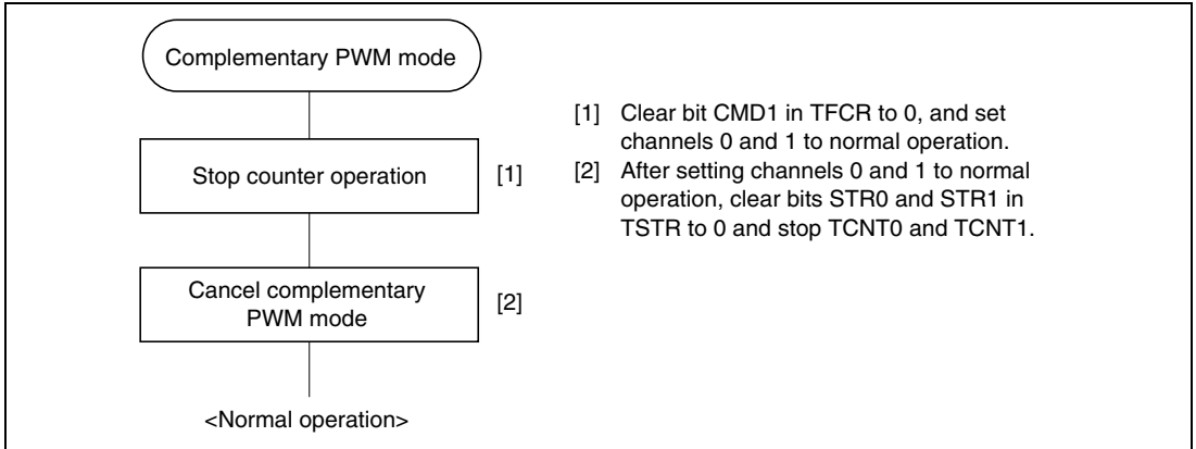
Figure 13.30 Canceling Procedure of Complementary PWM Mode
