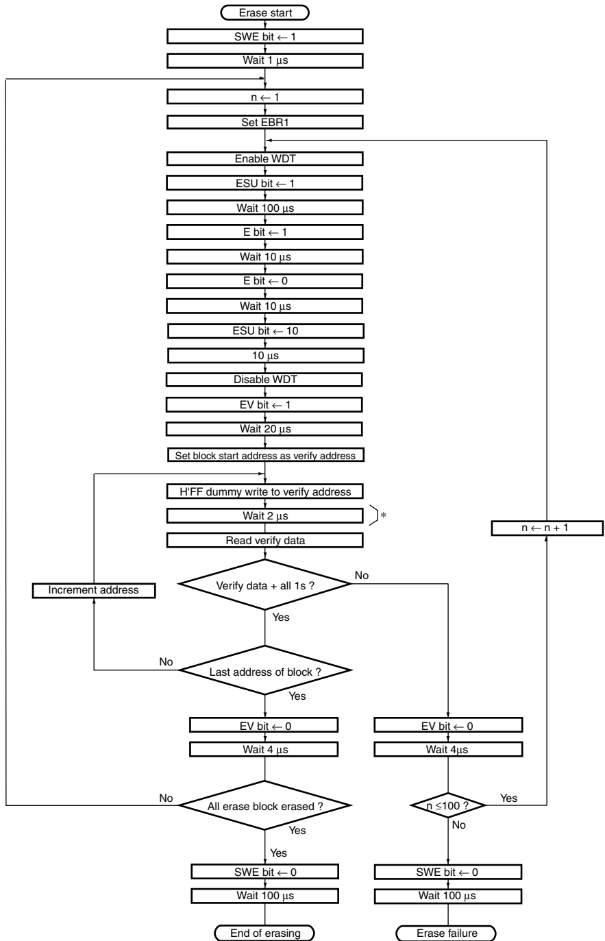
Figure 7.4 Erase/Erase-Verify Flowchart
