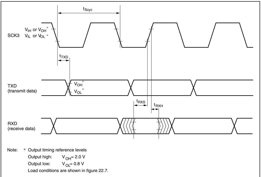
Figure 22.6 SCI Input/Output Timing in Clocked Synchronous Mode
