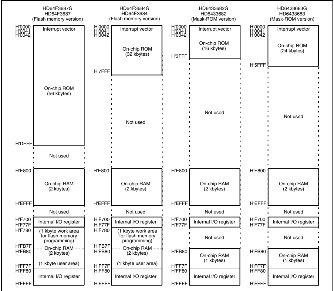
Figure 2.1 Memory Map (1)
