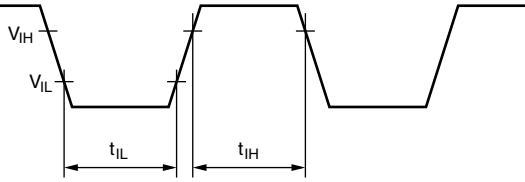
Figure 22.3 Input Timing
