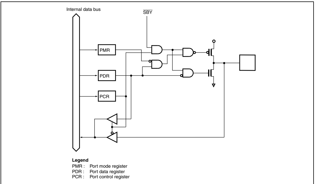
Figure B.7 Port 2 Block Diagram (P24, P23)
