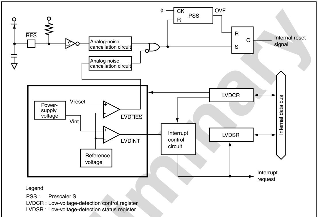
Figure 19.1 Block Diagram of Power-On Reset Circuit and Low-Voltage Detection Circuit
