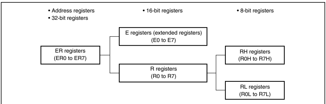
Figure 2.3 Usage of General Registers
