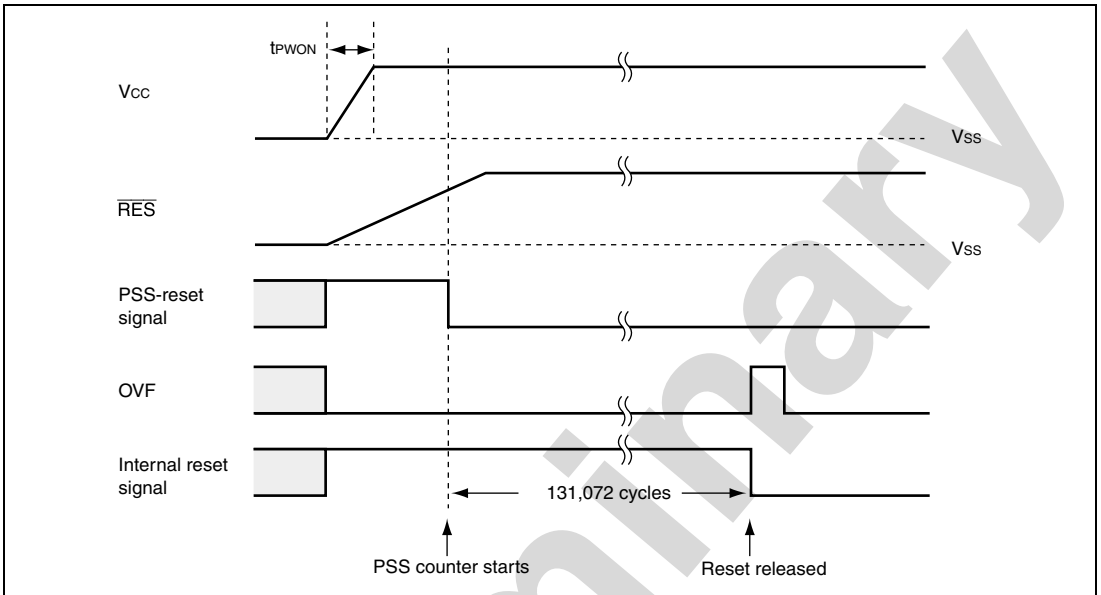
Figure 19.2 Operational Timing of Power-On Reset Circuit
