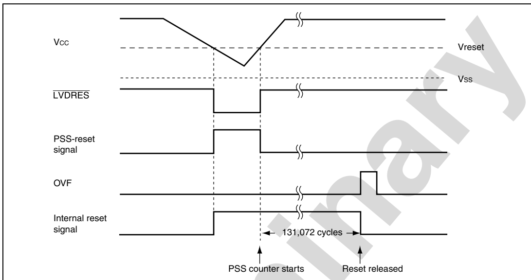
Figure 19.3 Operational Timing of LVDR
