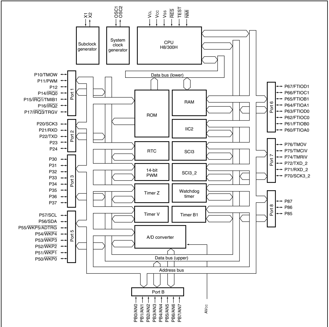
Figure 1.1 Internal Block Diagram of H8/3687 Series of F-ZTAT™ and Mask-ROM Versions
