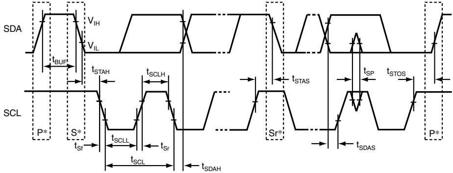
Figure 22.3 Input Timing
