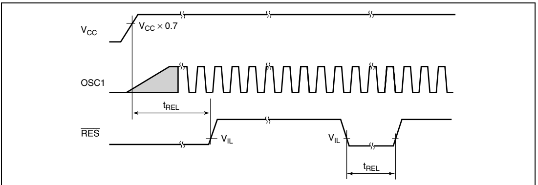
Figure 22.2 \overline{\text{RES}} Low Width Timing
