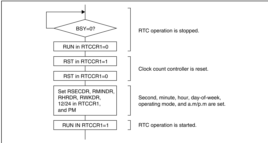
Figure 10.3 Initial Setting Procedure
