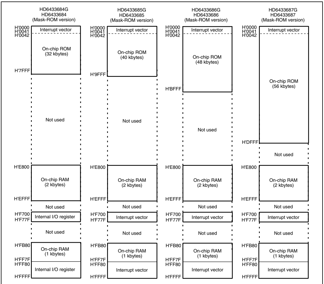
Figure 2.1 Memory Map (2)
