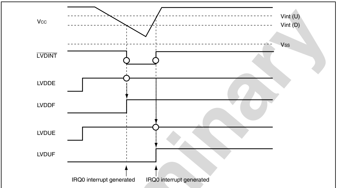
Figure 19.4 Operational Timing of LVDI
