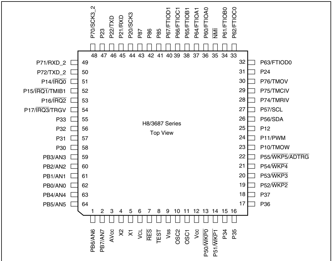
Figure 1.2 Pin Arrangement of H8/3687 Series of F-ZTAT™ and Mask-ROM Versions (FP-64E, FP-64A)
