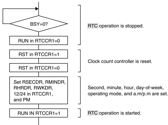
Figure 10.3 Initial Setting Procedure
